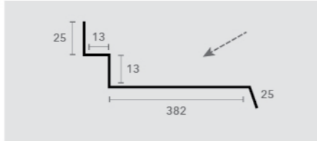
FASCIA SC18
