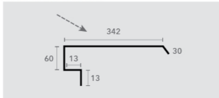
VALLEY SC18
